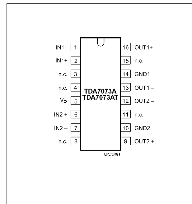
Pin Configuration
